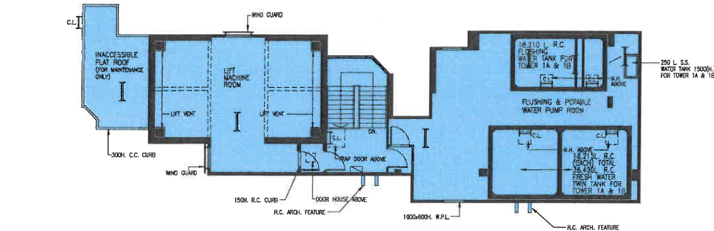
LIFT MACHINE ROOM PLAN (TOWER 1A & 1B)
